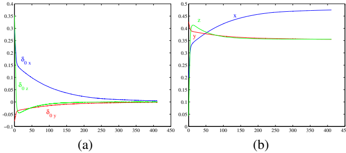
Fig. 6. V = kM\delta_f : time evolution of the image feature \delta_0 = R\delta (a), and of the pose \xi (b) for a real experiment.
