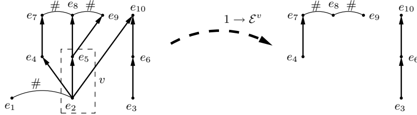
Figure 3: An event structure \mathcal{E} and a configuration v of \mathcal{E} . The future of v = \{e_2, e_5\} is shown on the right.
