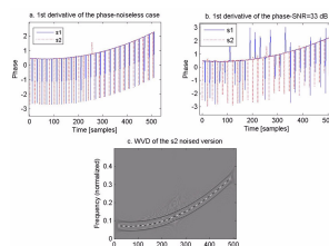
Fig. 4. Complementarity of time-frequency and time-phase information
