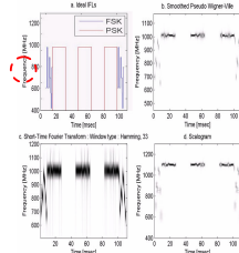
Fig. 1. Several TFRs of a mixed signal
