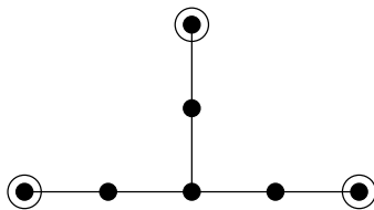
Figure 1: Graph containing an asteroidal triple
