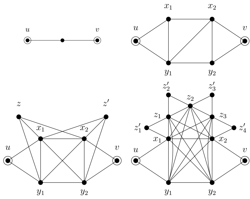
Figure 2: Examples of strong paths
