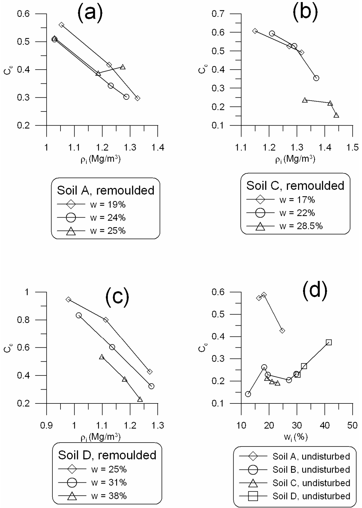
Fig. 7. Compression index ( C_c ) at various initial dry bulk densities ( \rho_i ) and initial water contents ( w_i ).
