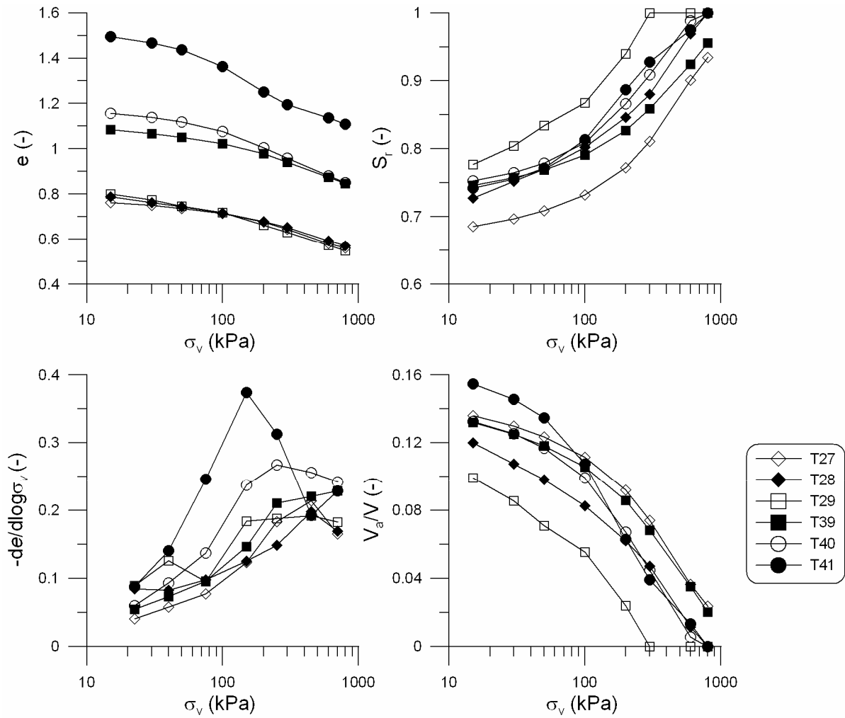
Fig. 6. Compression tests of soils C and D for 30 – 60 cm layer. Void ratio ( e ), degree of saturation ( S_r ), -de/d\log\sigma_v , and air content ( V_a/V ) versus logarithm of vertical stress ( \sigma_v ).
