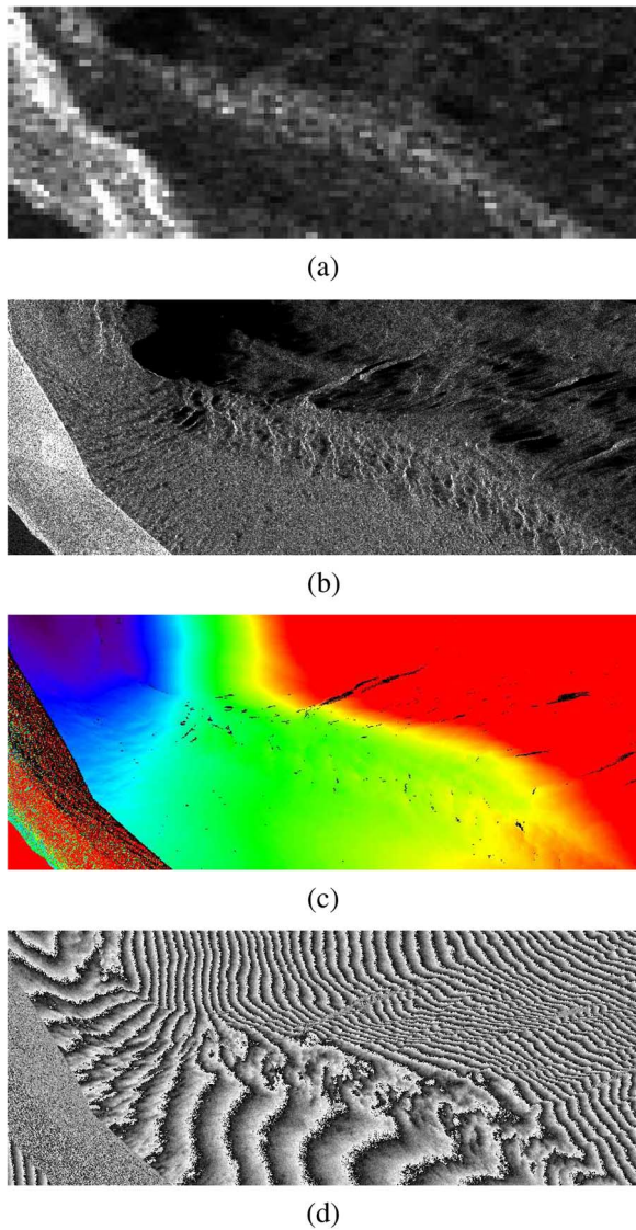
Fig. 4. Mer-de-glace glacier ( 840 \times 340 pixels). (a) ERS-1 five-look amplitude. (b) Simulated one-look TerraSAR-X amplitude. (c) Elevation image in TerraSAR-X slant range geometry. (d) Simulated one-look TerraSAR-X phase.
