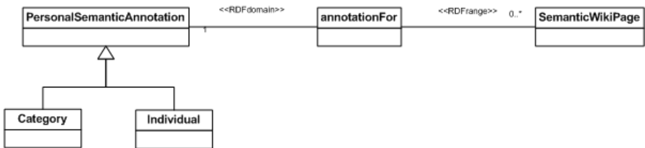
Figure 4: Personal Semantic Annotation Data Model
