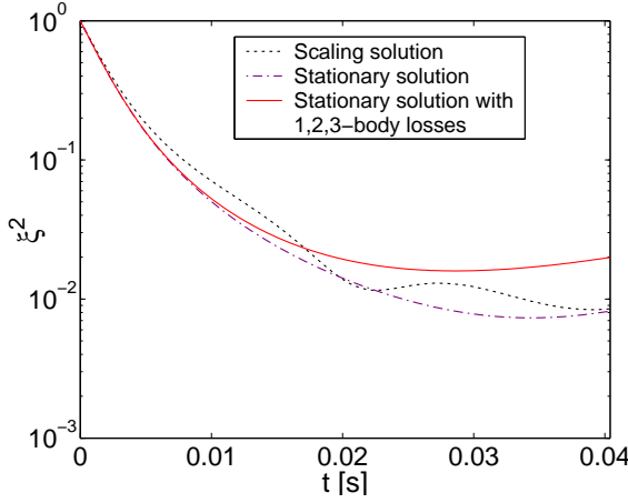
Fig. 11. Spin squeezing as a function of time in two small Rb condensates. Black dotted line: scaling solution based on (91). Violet dash-dotted line: stationary calculation without losses. Red solid line: stationary calculation with losses. Parameters: K_1^{(a)} = K_1^{(b)} = 0.01\text{s}^{-1} , K_2^{(a)} = 0 , K_2^{(b)} = 119 \times 10^{-21}\text{m}^3\text{s}^{-1} [24], K_3^{(a)} = 6 \times 10^{-42}\text{m}^6\text{s}^{-1} [26]. The other parameters: \bar{N}_a = \bar{N}_b = 10^3 , \omega_{x,y} = 2\pi \times 11.82\text{ Hz} , \omega_z = 2\pi \times 2\text{ kHz} , m=87\text{ a.m.u.} , a_{aa} = 100.44 r_B , a_{bb} = 95.47 r_B , a_{ab} = 98.09 r_B , r_B is the Bohr radius. \chi = 0.213\text{s}^{-1} , \tilde{\chi} = 2.763 \times 10^{-3}\text{s}^{-1} .
