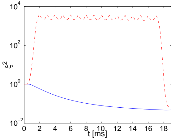
Fig. 9. Spin squeezing as the two Rb condensates are separated and put back together after an interaction time of about 15 ms. Red dashed line: Spin squeezing obtained from the definitions (10)-(12) of the spin operators explicitly including the overlap between the clouds. Blue solid line: extracted spin squeezing based of the “instantaneous modes” (42)-(43). Parameters as in Fig.8.
