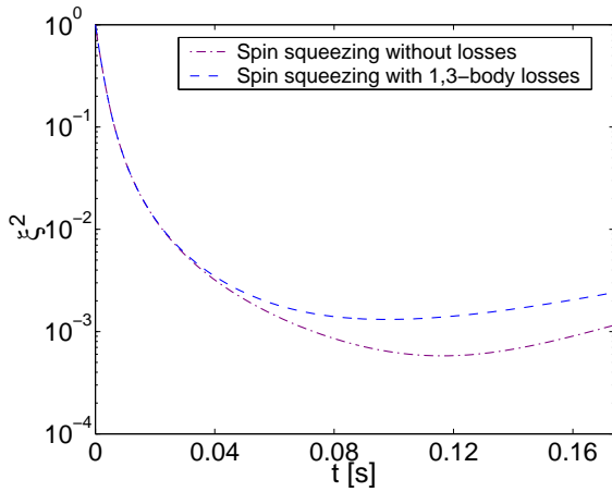
Fig. 7. Spin squeezing with and without losses in a bimodal Na condensate from the stationary two-mode model. Violet dash-dotted line: without losses. Blue dashed line: with one and three-body losses. Optimized parameters: \bar{N}_a = \bar{N}_b = 4 \times 10^4 , \omega = 2\pi \times 183 Hz, m=23 a.m.u., a_{aa} = a_{bb} = 51.89 r_B , a_{ab} = 48.25 r_B , r_B is the Bohr radius. \chi = 5.517 \times 10^{-3} \text{s}^{-1} , \tilde{\chi} = 0 . Particle losses: K_1^{(a)} = K_1^{(b)} = 0.01 \text{s}^{-1} , K_2^{(a)} = K_2^{(b)} = 0 , K_3^{(a)} = K_3^{(b)} = 2 \times 10^{-42} \text{m}^6 \text{s}^{-1} [27].
