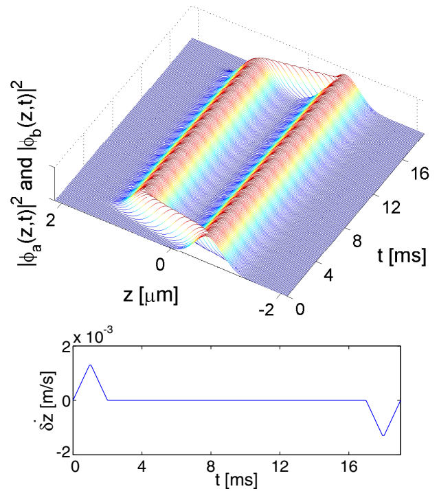
Fig. 8. (Top) |\phi_a(z,t)|^2 and |\phi_b(z,t)|^2 in arbitrary units as the clouds are separated and put back together after an interaction time of about 15 ms. The harmonic potential for the a -component does not move, while that for the b -component is shifted vertically with a speed \delta z . The distance between the two trap centers when they are separated is \delta z = 4\sqrt{\hbar/M\omega_z} . (Bottom) variation in time of \delta z . Parameters: \bar{N}_a = \bar{N}_b = 5 \times 10^4 , \omega_{x,y} = 2\pi \times 2.31 Hz, \omega_z = 2\pi \times 1 kHz, m=87 a.m.u., a_{aa} = 100.44 r_B , a_{bb} = 95.47 r_B , a_{ab} = 98.09 r_B , r_B is the Bohr radius. No particle losses.
