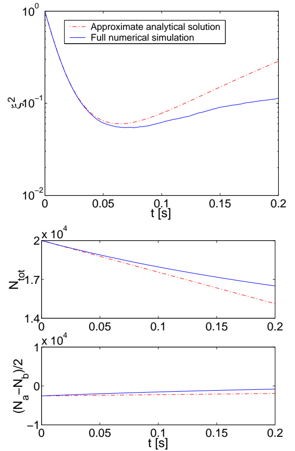
Fig. 13. (Top) Spin squeezing with two-body losses in a bimodal Rb condensate as a function of time in breathe-together configuration. Blue solid line: exact numerical simulation with 4000 realizations. Red dash-dotted line: analytical solution with constant loss rate approximation. (Bottom) Corresponding total number of particles and \langle S_z \rangle as a function of time. Parameters: \bar{N}_a = 7432 , \bar{N}_b = 12568 , \chi = 5.392 \times 10^{-3} \text{s}^{-1} , \tilde{\chi} = 1.386 \times 10^{-3} \text{s}^{-1} , v = 13.850 \text{s}^{-1} . The other parameters are the same as in Fig.12.
