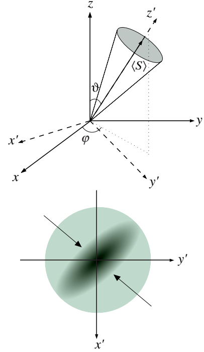
Fig. 1. (Top) average spin. (Bottom) variance of the the spin components in the plane orthogonal to the mean spin.
