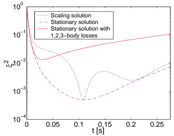
Fig. 10. Spin squeezing as a function of time. (Top) comparison between a dynamical calculation and a stationary calculation. Blue solid line: extracted spin squeezing in 3D. Black dotted line: 2D scaling solution based on (91). Violet dash-dotted line: stationary calculation in 3D without losses. Red solid line: stationary calculation in 3D with losses. Spin squeezing progresses more slowly in the dynamical calculation than in the stationary calculation. (Bottom) long time behavior. Black dotted line: scaling solution. Violet dash-dotted line: stationary calculation without losses. Red solid line: stationary calculation with losses. Parameters: \chi = 5.003 \times 10^{-3} \text{s}^{-1} , \tilde{\chi} = 1.342 \times 10^{-4} \text{s}^{-1} , K_1^{(a)} = K_1^{(b)} = 0.01 \text{s}^{-1} , K_2^{(a)} = 0 , K_2^{(b)} = 119 \times 10^{-21} \text{m}^3 \text{s}^{-1} [24], K_3^{(a)} = 6 \times 10^{-42} \text{m}^6 \text{s}^{-1} [26]. The other parameters are as in Fig.8.
