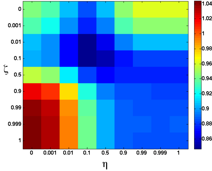
Figure 3: A heat plot of performance for a range of kernel parameter choices, \eta and \zeta , using the MovieLens dataset.
