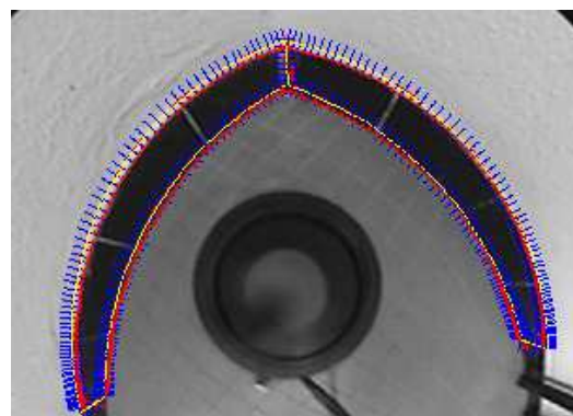
Fig. 8. Tracking plinths: red points correspond to the points p extracted by the ME algorithm along the normals to the previous 3D model projection (in blue). Forward projection of the model for a given pose is displayed in yellow.
