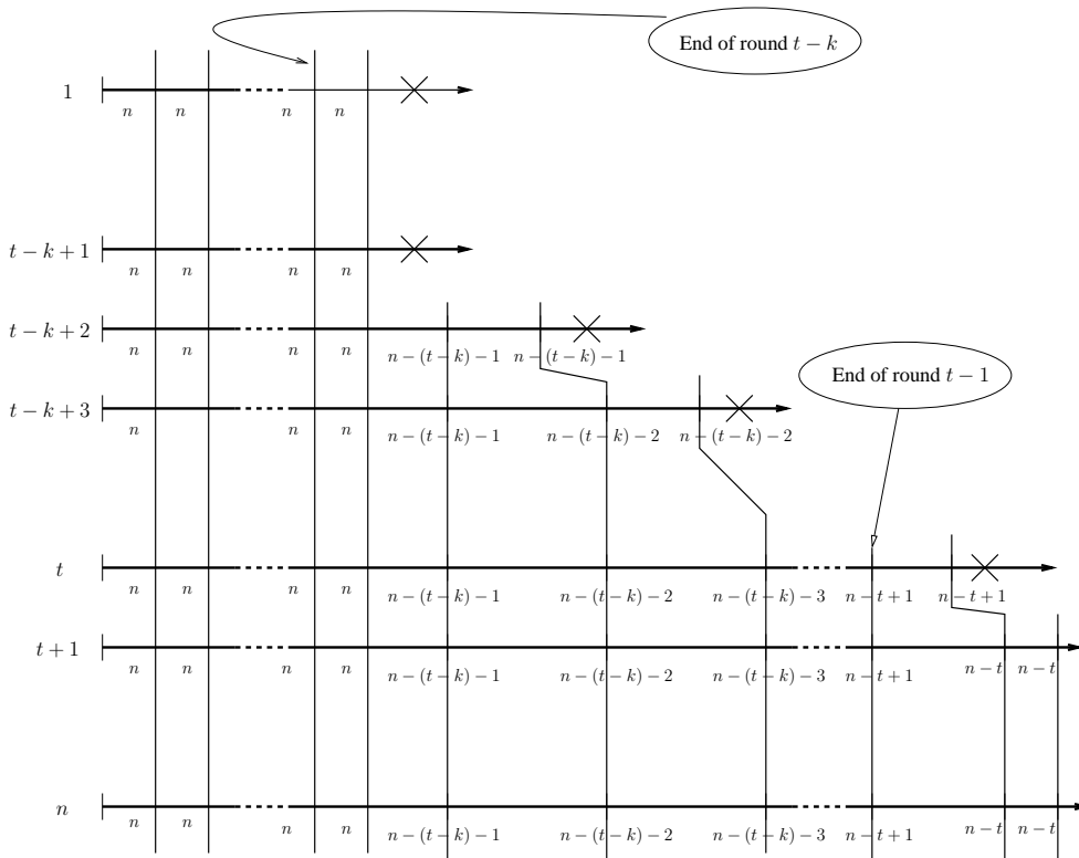
Figure 12: Run R_k
