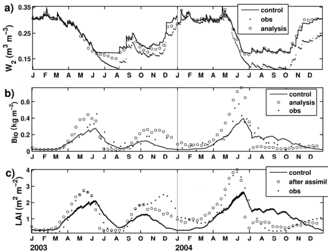
Figure 4.- Analysis of a) the root zone soil moisture (circles) and b) vegetation biomass, using the simplified 1D-VAR method and a fixed wilting point for 2003 to 2004 over the SMOSREX experimental site. c) LAI before and after the assimilation. For comparison purposes, analysed values are superimposed over the in-situ observations (points) and the model basic estimations (solid line).
