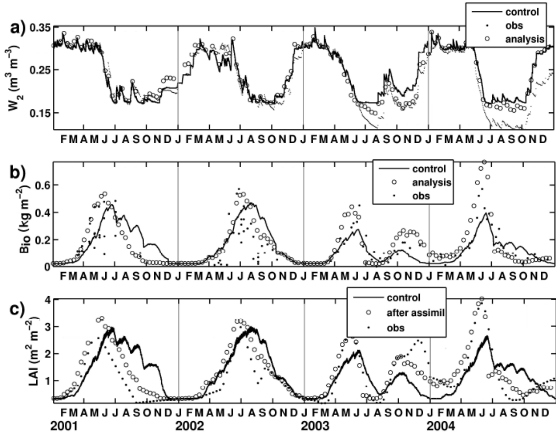
1 2 Figure 3.- Analysis of a) the root zone soil moisture (circles) and b) vegetation biomass, 3 using the simplified 1D-VAR method and a dynamical correction of the wilting 4 point for 2001 to 2004 over the SMOSREX experimental site. c) LAI before and 5 after the assimilation. For comparison purposes, analysed values are superimposed 6 over the in-situ observations (points) and the model basic estimations (solid line).
