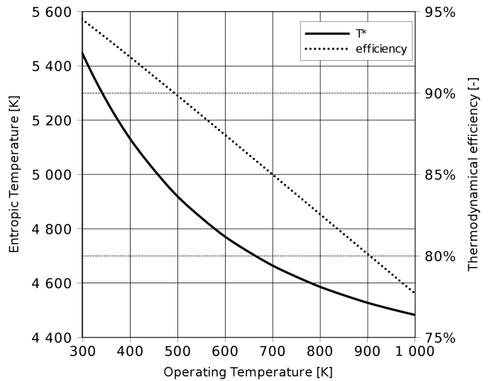
Fig. 4. Entropic temperature T^* and efficiency \eta .
