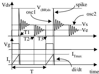
Figure 7 : parasitic oscillations
