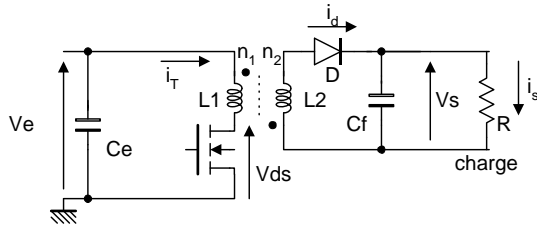
Figure 3 : simplified schematic
