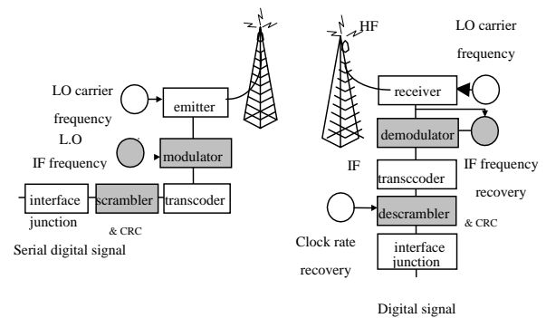
Fig 1 : Digital transmission block diagram
