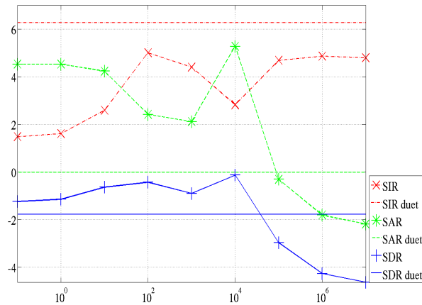
Figure 3: SDR, SIR, SAR of the proposed iterative algorithm and DUET as function of the penalty factor \lambda (log scale).
