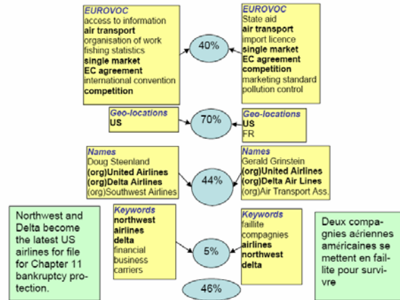
Figure 4. Example of the similarity calculation for an English and a French cluster. The overall similarity for these two clusters, based on the linear combination of four different vectors, is 0.46.
