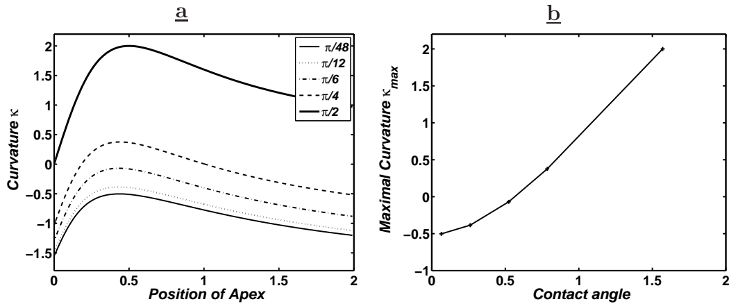
FIG. C.4: Effect of the contact angle on the curvature.
