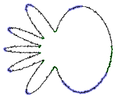
(c) GMC: minima/maxima \nu = 4
