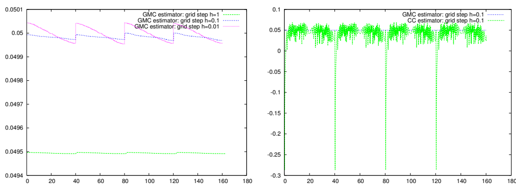
(a) Circle radius R = 20 with \epsilon_1 = 1e - 6 , \epsilon_{0.1} = 1e - 7 , \epsilon_{0.01} = 1e - 8
