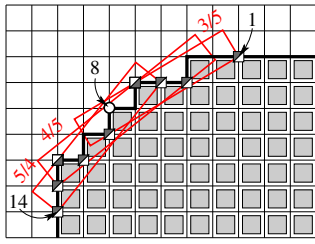
Fig. 4. Estimation of the possible tangent directions of shapes that are digitized as the black pixels. On the left, the maximal segments surrounding point C_8 are displayed with their slope. Each one defines possible tangent directions for their included points. It is enough to consider points that are extremities of a maximal segment to define a piecewise linear tangent representation of a contour which stays within the boxes. The bounds a and b are displayed for two of these points on the right.
