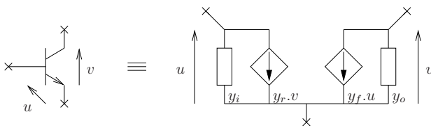
Figure 3: y -parameter representation of a transistor.
