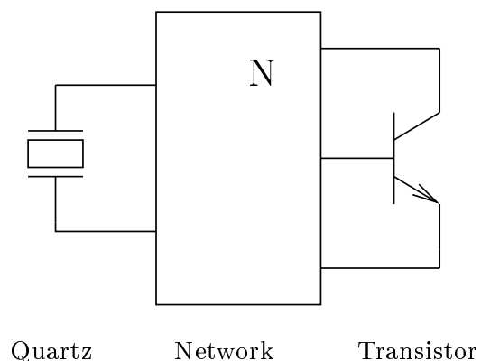
Figure 1: 5-terminal representation of a quartz crystal oscillator.
