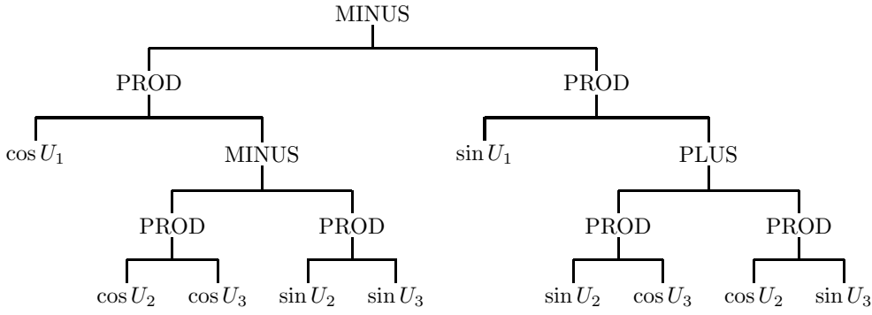
Fig. 4: Binary tree of cosinus
