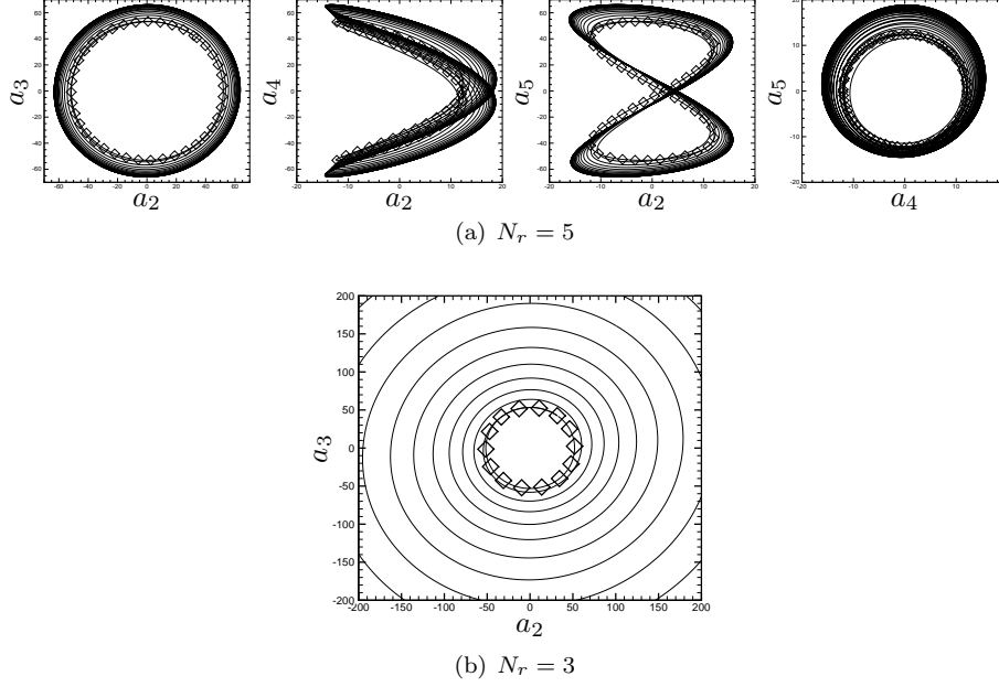
Figure 4: Comparison of the projected (NS: \diamond ) and the predicted (Standard pressure ROM: \text{—} ) limit cycles over 1000 vortex shedding periods.
