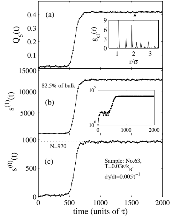
Figure 1: Time-dependence of different characteristics computed for a single sheared sample with the strain rate \dot{\gamma} = 0.005\tau^{-1} at the temperature T = 0.03\epsilon/k_B : (a) Global orientational bond-order parameter Q_6(t) . Inset: radial distribution of particles formative the ordered cluster structures. It is defined for the moment indicated by arrow. Pronounced peaks of radial distribution appear at the distances \sim \sigma n^{1/2} , n = 1, 2, 3, \dots is the number of a peak, that is typical for FCC structures. (b) Number of solidlike particles s^{(1)}(t) . Inset shows the same in logarithmic scale. (c) Number of clusters s^{(0)}(t) .
