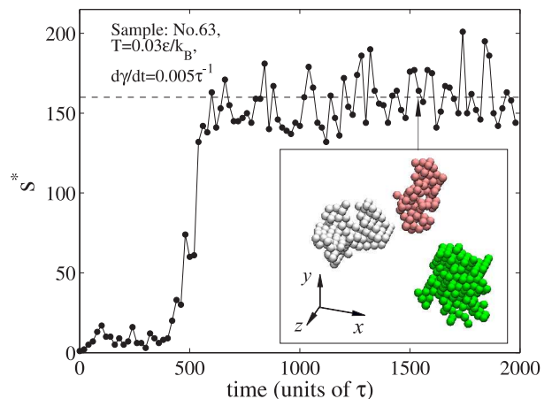
Figure 5: (Color online) Main: Size of the largest cluster versus time. Broken line corresponds to the value 160. The study sample is still the same as for the previous figures. Inset: Three largest clusters at the moment indicated by arrow. The sizes of the clusters are N_1 = 177 , N_2 = 130 and N_3 = 126 particles.
