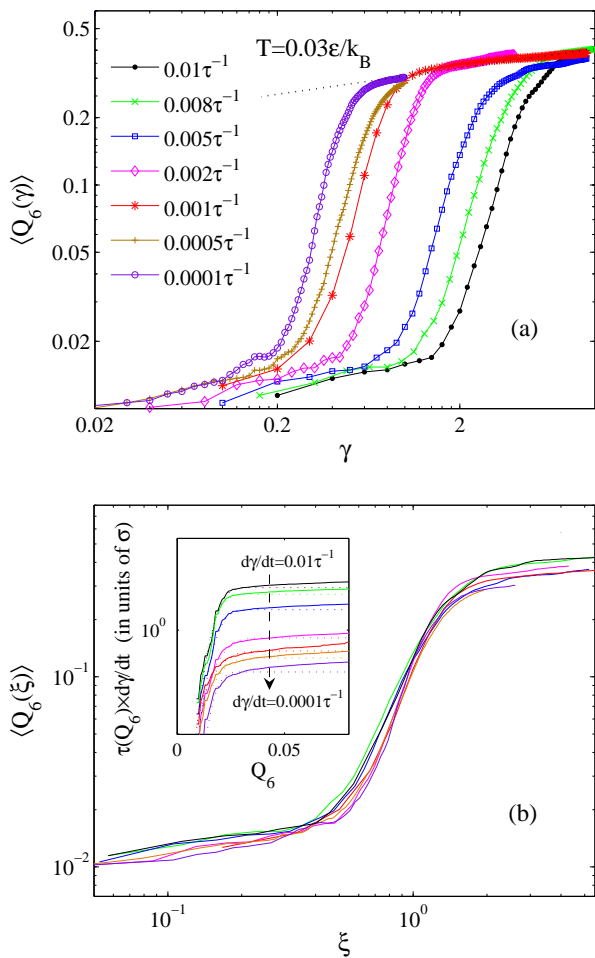
Figure 6: (Color online) (a) Orientational bond-order parameter of a sheared system (amorphous initially) versus strain. Each curve corresponds to a fixed strain rate \dot{\gamma} \in [0.0001, 0.01]\tau^{-1} and is averaged over results obtained for at least 50 independent samples, which were sheared under the same conditions at a temperature T = 0.03\epsilon/k_B . (b) Main: Orientational bond-order parameter versus rescaled transition strains \xi = \gamma/\gamma_n . Inset: Mean first passage time distributions multiplied by the corresponding strain rates. The solid lines are results of simulations, the dotted lines present the fits to Eq. (3).
