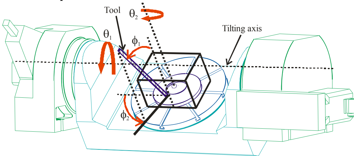
Figure 7: Draw of the tilting table: the tool orientation is defined by two angles ( \phi_1, \phi_2 ) relative to frame R_t linked to the tilting table. The orientation angles ( \theta_1, \theta_2 ) of the tilting table are defined relative to frame R_b fixed to the base of the VERNE machine
