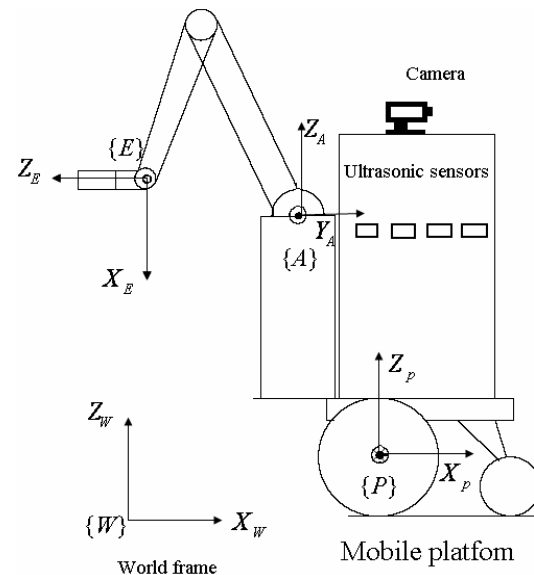
Figure 1. Mobile arm manipulator
