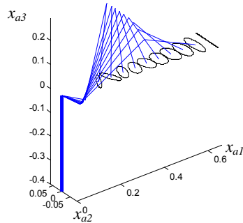
Figure 4. Manipulability ellipses
