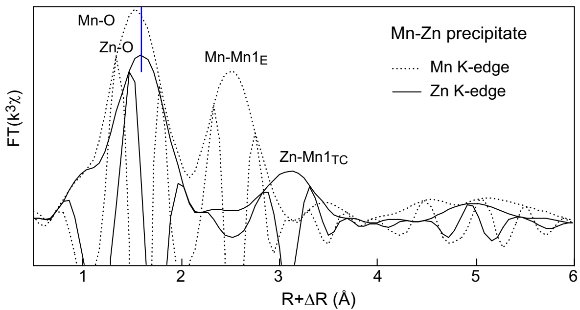
Fig. EA-7: Fourier transform of the EXAFS spectra for the Mn-Zn precipitate at the Mn and Zn K-edges. The average Mn-O and Zn-O EXAFS distances ( R values) are 1.90 Å and 2.00 Å, respectively.
