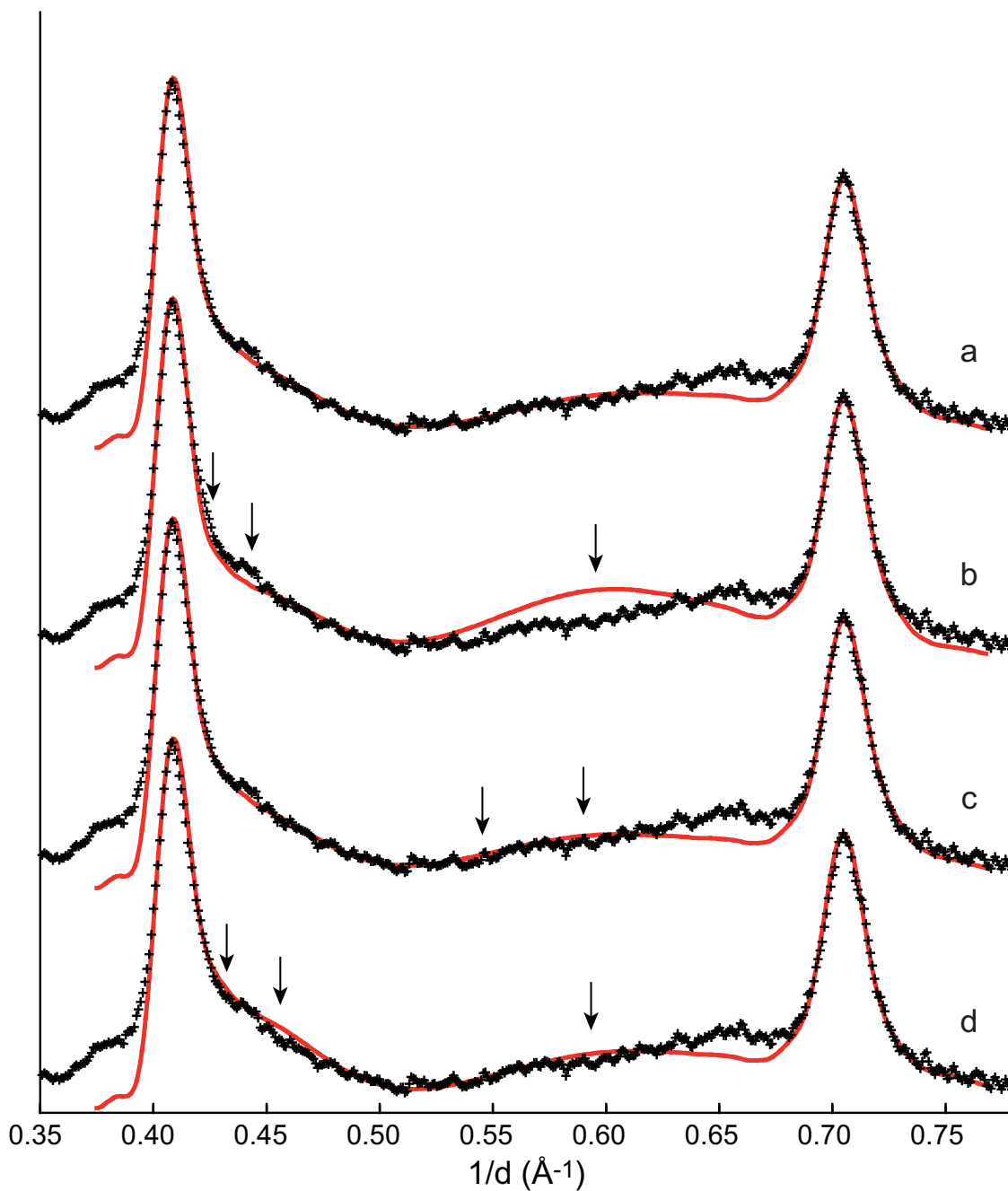
Fig. EA-6: Simulations of the [20,11] and [02,31] X-ray scattering bands (C-centered layer cell, black crosses). Small but significant misfits between experimental and calculated patterns are pointed out with arrows. Intensities (red lines) were calculated with a turbostratic layer stacking (no interlayer correlation). (a) Optimal model (Table 1; Figs. 8 and EA-5); R_{wp} = 3.49\% . (b) Model with ^{IV}Zn (Zn2) in (0, 0, 1.97 Å), instead of (0, 0, 1.77 Å) in the optimal fit, so as to increase the Zn-O bond length from 1.82 Å (Table 2) to 1.91 Å. Coordinated H_2O molecules (O4) were moved from (0, 0, 3.70 Å) to (0, 0, 3.90 Å); R_{wp} = 3.92\% . (c) Model with ^{VI}Zn (Zn1) in (0, 0, 2.30 Å), instead of (0, 0, 2.20 Å) in the optimal fit so as to decrease the sum valence of Zn1 from 2.3 (Table EA-1) to 2.0. Coordinated H_2O molecules (O2) were moved from (-0.333, 0, 3.45 Å) to (-0.333, 0, 3.65 Å); R_{wp} = 3.55\% . (d) Model with Ca in (-0.333, 0, 3.60 Å), instead of (-0.410, 0, 3.60 Å) and equivalent positions in the optimal fit; R_{wp} = 3.51\% . Unless specified, all parameters used in calculations are those of the optimal model.
