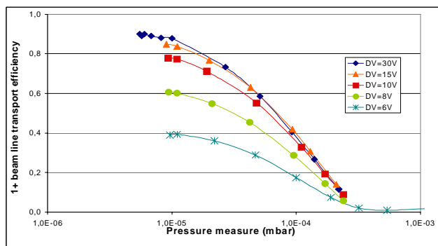
Figure 10: Gas pressure effect on the 1+ beam line efficiency.
