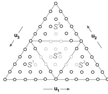
Figure 9: control points known from the boundary curves and their cross-boundary tangents, ensuring pairwise G^1 continuity between macro-patches
