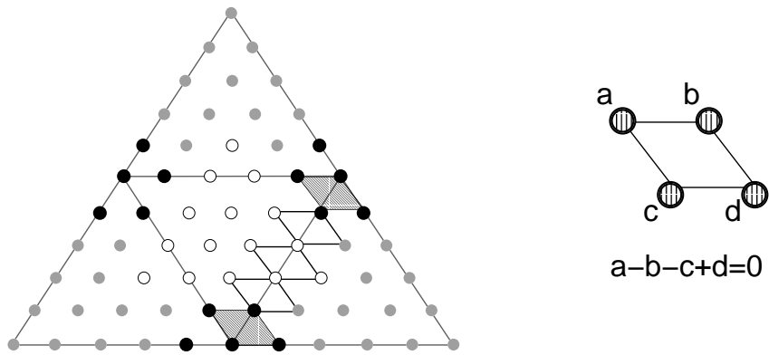
Figure 12: C^1 -conditions between two adjacent quintic Bézier patches inside one macro-patch.
