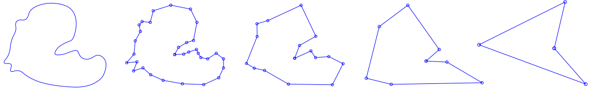
Figure 2: From left to right, a B-spline curve defined by 32 control points, its control polygon (level 5), the control polygons of its coarse approximations at levels 4, 3 and 2.
