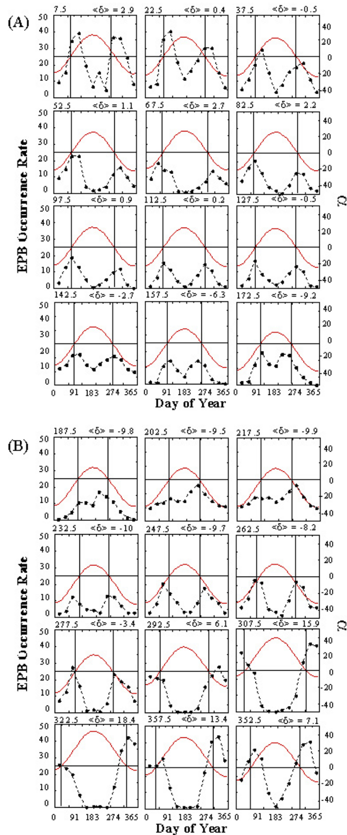
Fig. 3. Values of \alpha and measured rates of EPB occurrence plotted as functions of day of the year. Vertical lines indicate days when \alpha = 0^\circ . Central longitudes and average declinations are noted at the top of each panel. Segment A (B) summarizes data acquired in the 0^\circ to 180^\circ ( 180^\circ to 360^\circ ) longitude range.
