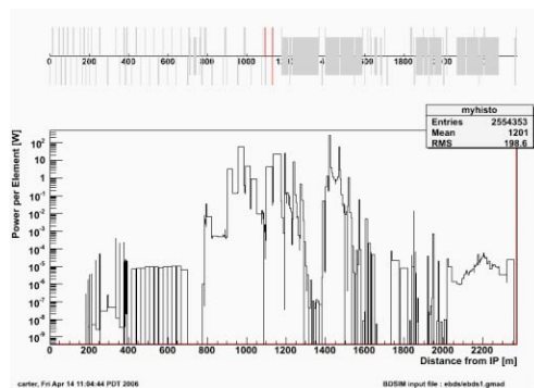
Figure 4: Power deposition along the ILC beam delivery system
