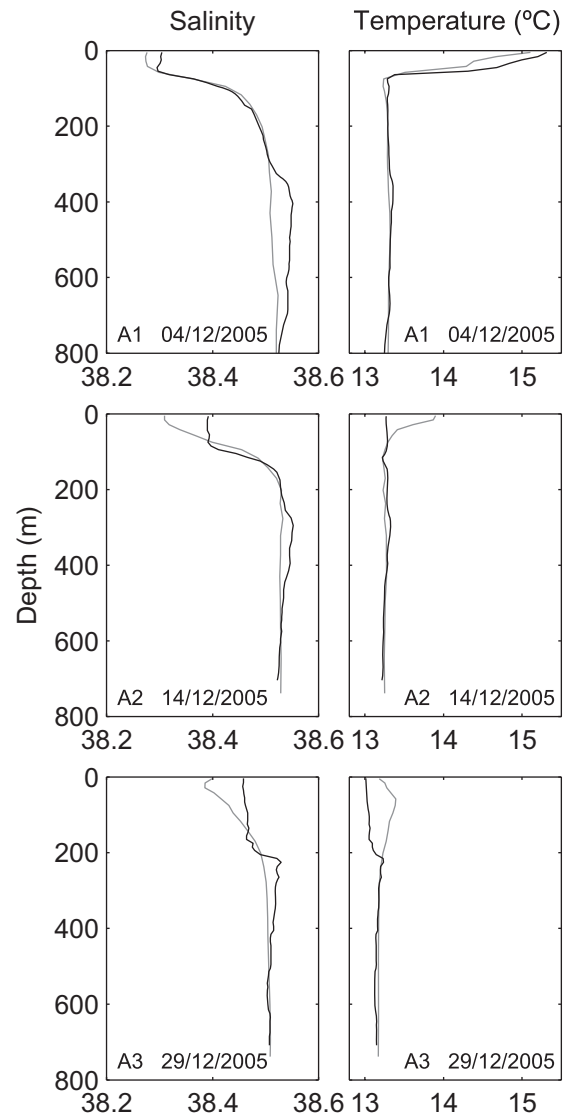
Fig. 10. Comparison between model temperature and salinity profiles (grey line) and those measured by Argo floats (black line). The date of each profile is indicated and its location is shown in Fig. 1.
