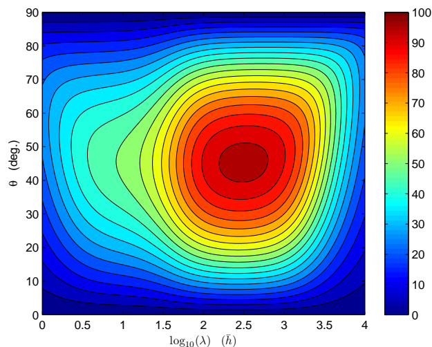
Fig. 8. (a) The steady-state amplitude ratio ( |T_{vb}| ) between transverse velocity ( \Delta v ) and bedrock topography ( \Delta b ) in the shallow ice stream approximation (Eq. 22). Surface slope is 0.002 and the slip ratio is 99.
