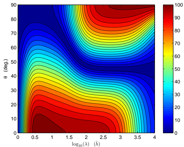
Fig. 7. (b) The steady-state amplitude ratio ( |T_{ub}| ) between longitudinal surface velocity ( \Delta u ) and bedrock topography ( \Delta b ) (Eq. 75 in Gudmundsson, 2003). The shape of the same transfer function for the same set of parameters, but based on the shallow ice stream approximation, is shown in Fig. 7a.
