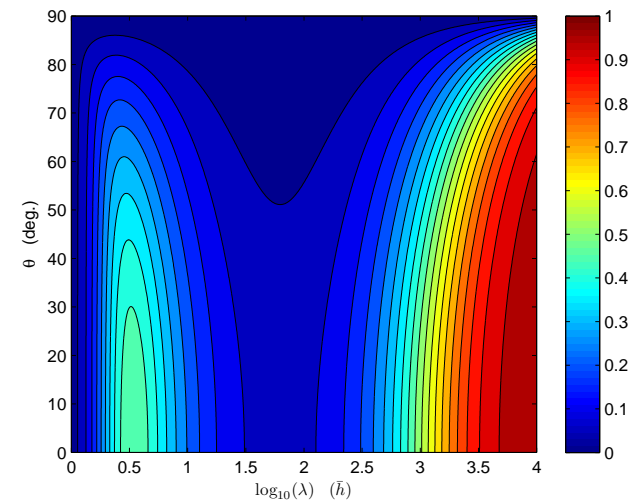
Fig. 6. (b) The FS amplitude ratio between surface and bedrock topography ( |T_{sb}| ) from Eq. (75) in Gudmundsson (2003). The shape of the same transfer function for the same set of parameters based on the SSTREAM approximation is shown in Fig. 6a.
