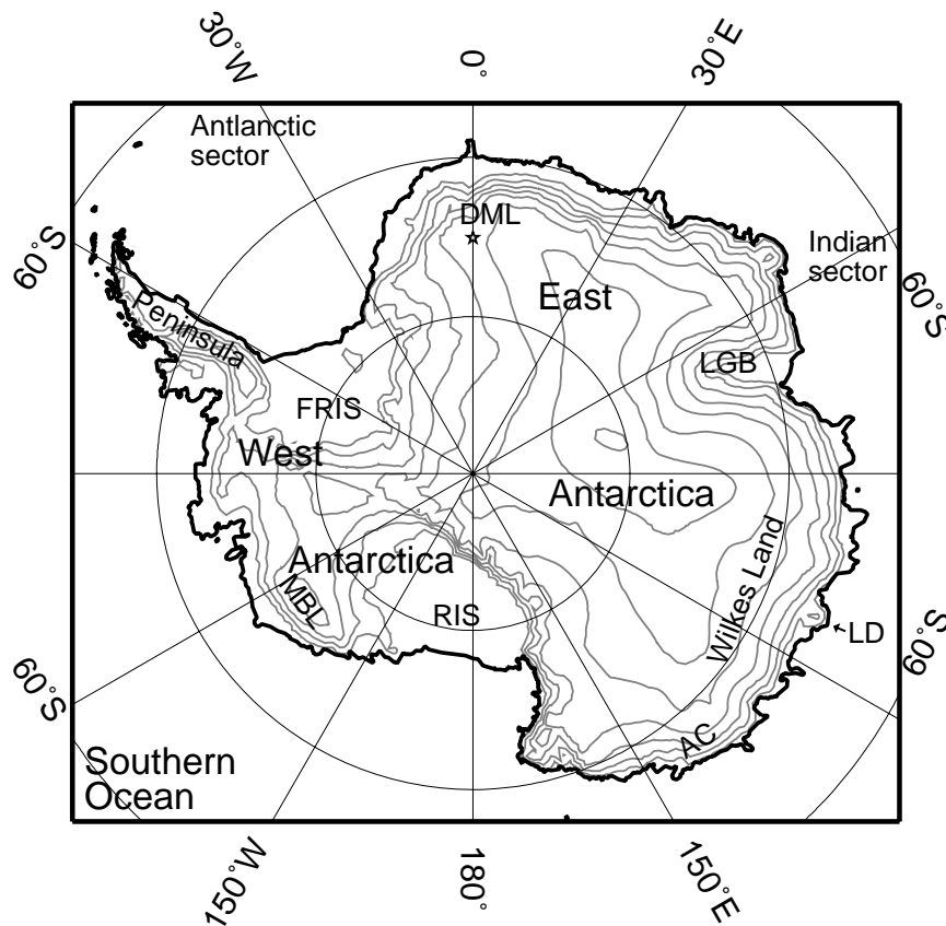
Fig. 2. Map of Antarctica. The star locate Kohonen Station. DML, LGB, LD, AC, RIS, MBL and FRIS denote Dronning Maud Land, Lambert Glacier Bassin, Law Dome, Adélie Coast, Ross Ice Shelf, Marie Byrd Land and Filchner-Ronne Ice Shelf, respectively.
