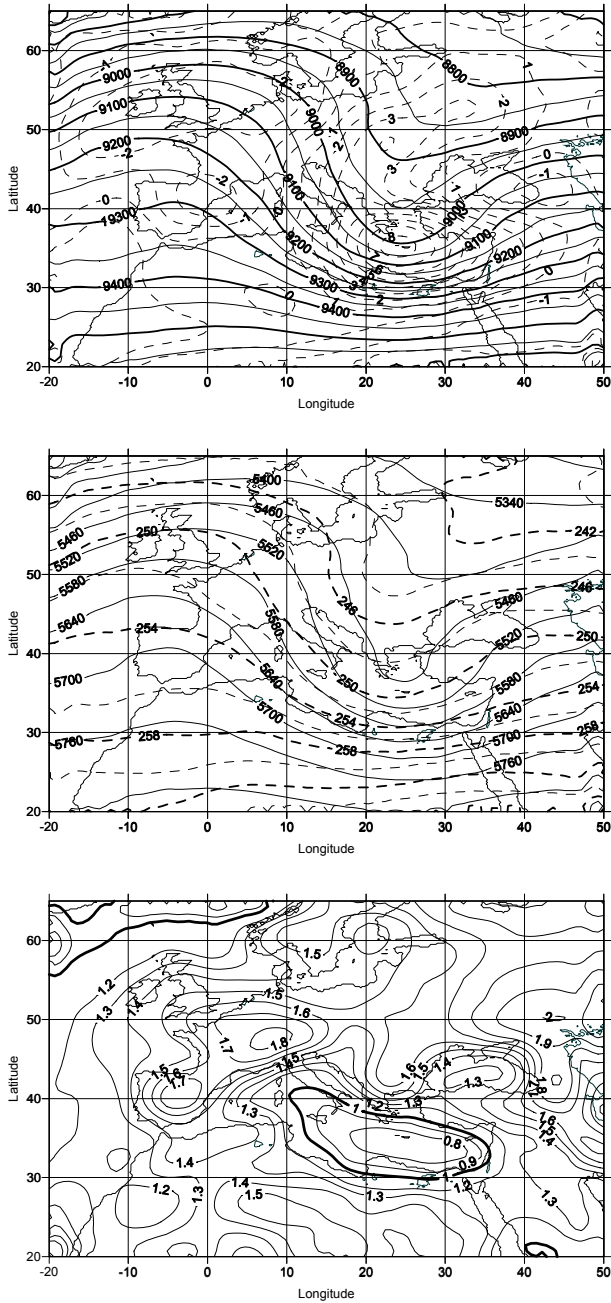
Fig. 3. Same as Fig. 2 but for D0.
