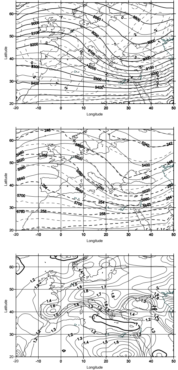
Fig. 4. Same as Fig. 2 but for D+2.
