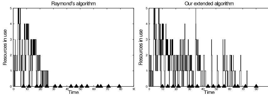
FIG. 4: Efficiency comparison of Raymond algorithm and our extension
