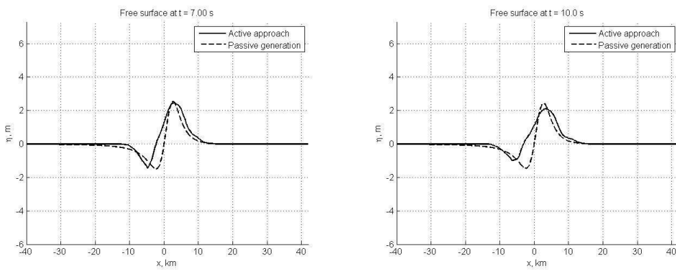
Fig. 6. Same as figure 4 for times t = 7 s and t = 10 s.
