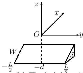
Fig. 1. Geometry of the source model. The fault has width W , length L , depth d and dip angle \delta .
