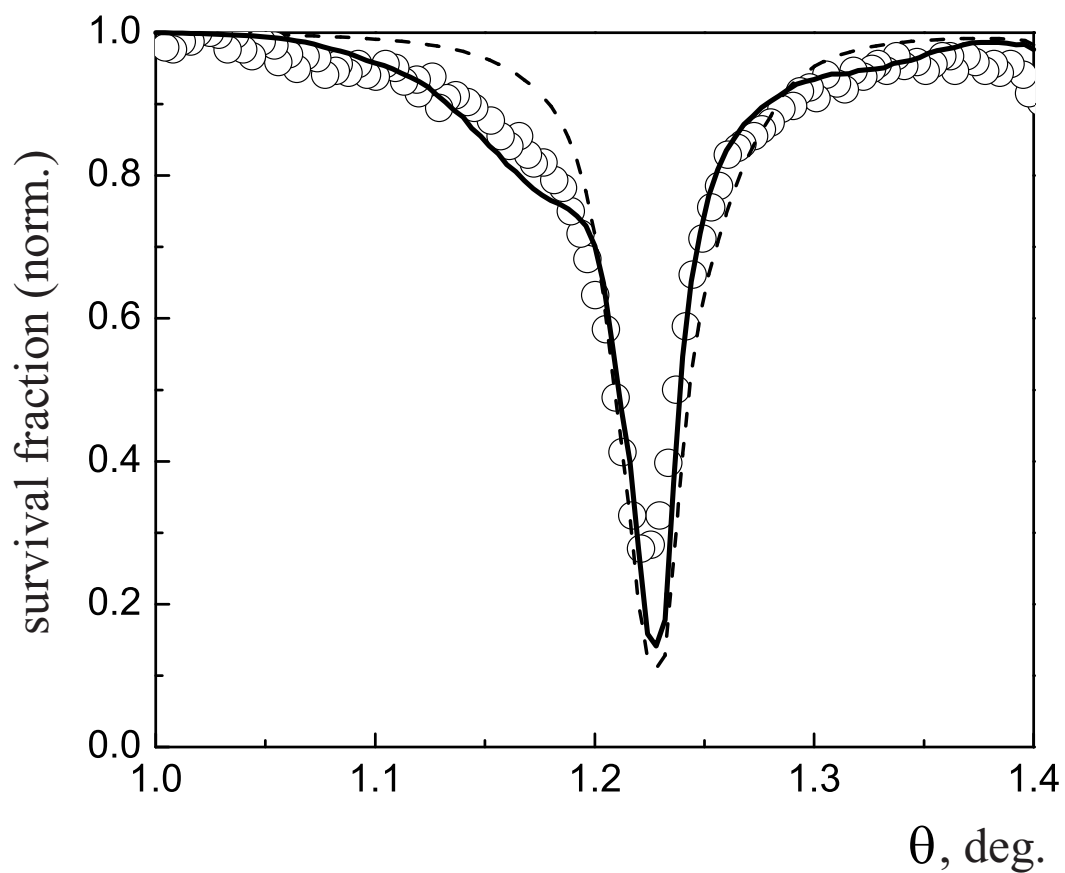
Fig. 3. Normalized survival fraction of 387.90 MeV/u \text{Ar}^{16+} ions passing through a 27 \mu\text{m} Si crystal. Solid line — calculations with 2p^2 : ^1D_2 - 2s2p : ^1P_1 mixing, dash line — calculations without 2s2p : ^1P_1 state. Experimental data (circles) are taken from [6].
