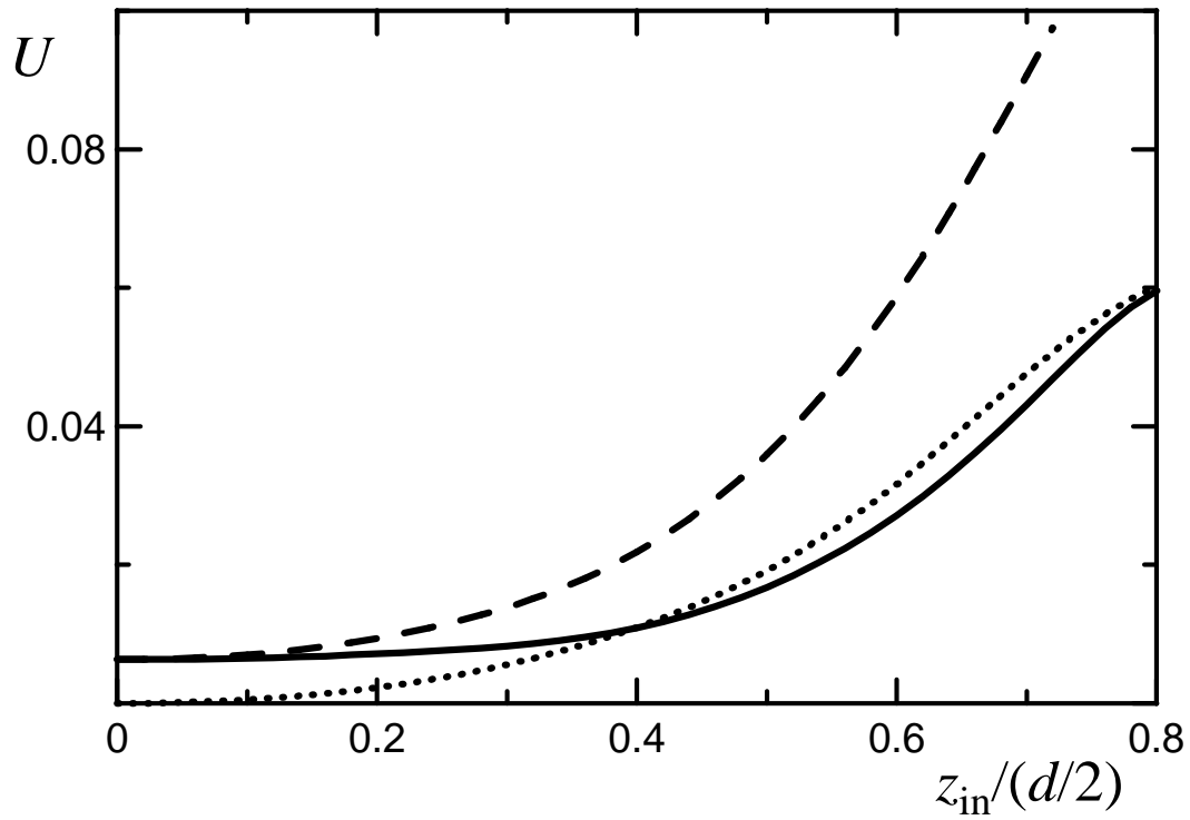
Fig. 1. Trajectory resolved differential yield of X-ray radiation from 423 MeV/u \text{Fe}^{24+} ions under RCE conditions at (k, l) = (2, -1) resonance in the directions of X axis (solid line), Y axis (dashed line) and Z axis (dotted line).
