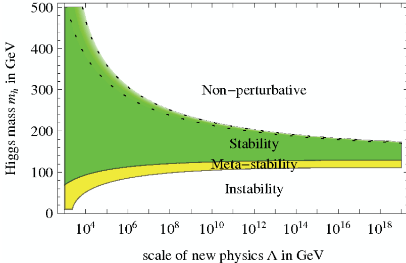
Figure 6: Bounds on the Higgs mass.
