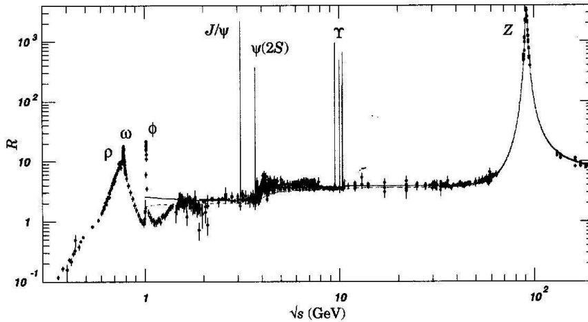
Figure 5: The ratio R of e^+ + e^- total cross section to hadrons normalised to that of e^+ + e^- \rightarrow \mu^+ + \mu^- as a function of the centre-of-mass energy.
