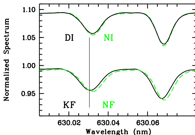
Fig. 3. The four observed spectra we used for the analysis of the [O I] 630 nm line. The Kurucz Flux spectrum, KF, and the Neckel Flux, NF, and Neckel Intensity, NI, spectra here plotted are the normalised spectra provided by Kurucz (2005a) and Neckel (1999) respectively; the Neckel Intensity, NI, is shifted up by 0.1 for clarity, while the Delbouille Intensity, DI, has been normalised and then shifted up by 0.1. The vertical line indicates the laboratory wavelength of the oxygen line. We recall that KF is corrected for gravitational redshift while NF is not, explaining the large wavelength differences between the two flux atlases
