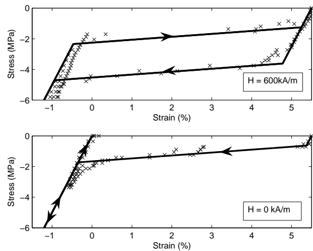
Fig. 1. Mechanical stress versus strain with and without a magnetic field for a cyclic charging (simulation: solid line, experimental results: cross points)
