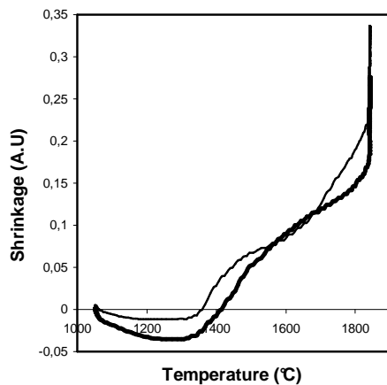
Fig.1. Densification curves, 15°C/min, dwell at 1830°C
