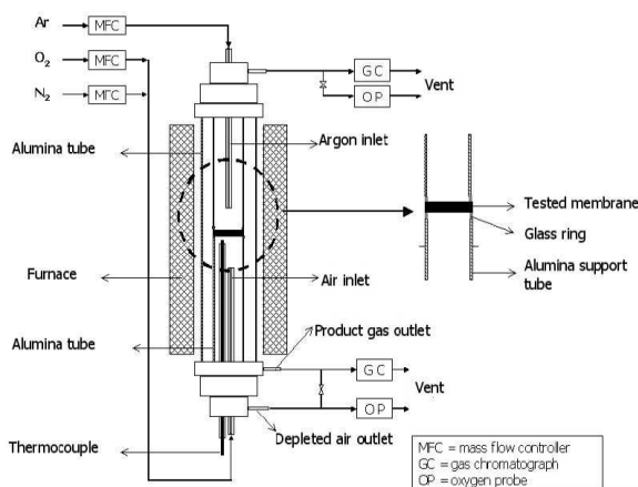
Figure 1: Schematic diagram of oxygen permeation flux measurements system
