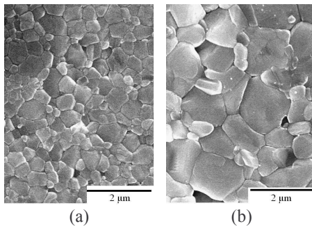
Figure 5: SEM micrographs of \text{La}_{0.8}\text{Sr}_{0.2}\text{Fe}_{0.7}\text{Ga}_{0.3}\text{O}_{3-\delta} sintered, (a) 1250°C for 2h and (b) 1350°C for 10h.
