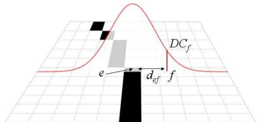
Figure 2: Distance weight for the well-detection criterion.
