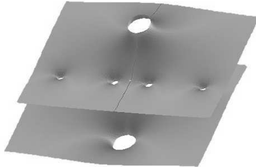
Figure 3: An element in the corresponding family of minimal surfaces. Computer image made by the author using J. Hoffman MESH software.
