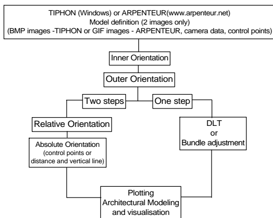
Figure 1. Overview of the current photogrammetric solutions available in TIPHON-ARPEITEUR
