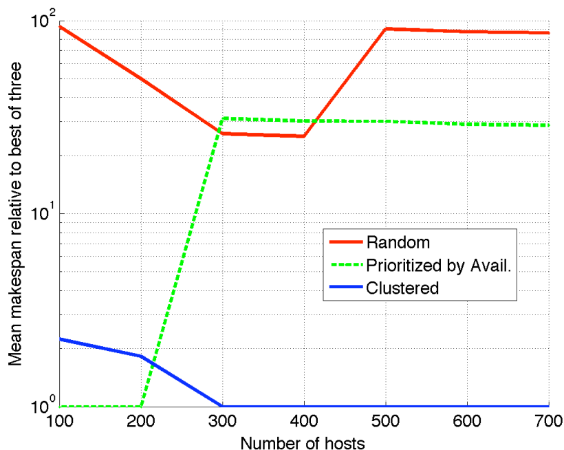
Figure 6: Performance of Barrier Synchron Application
