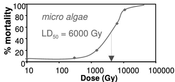
Figure 2: Micro algae mortality vs. radiation dose. The line is a guide to the eye.
