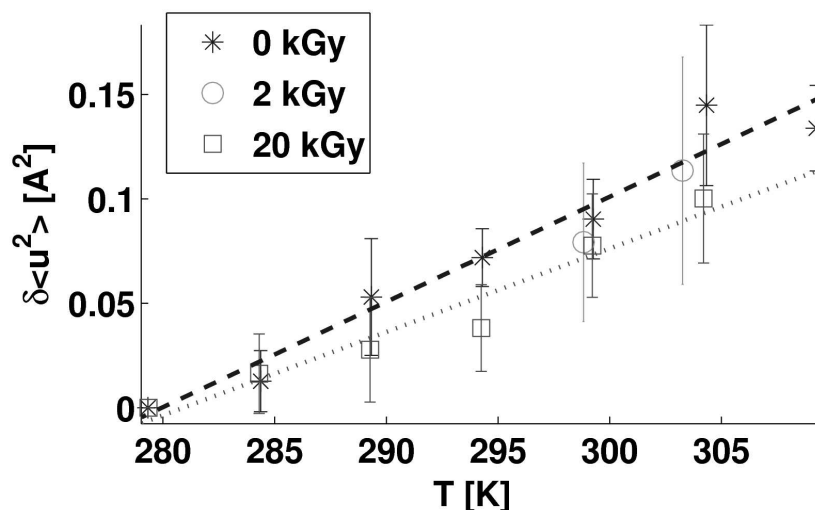
Figure 6: Micro algae mean square displacement temperature shift w.r.t. T=280 \text{ K} vs. integrated dose. Lines are linear fit to the curves in order to extract the associated resilience k . The \langle u^2 \rangle values at T=280 \text{ K} are around 1.4 \text{ \AA}^2 .
