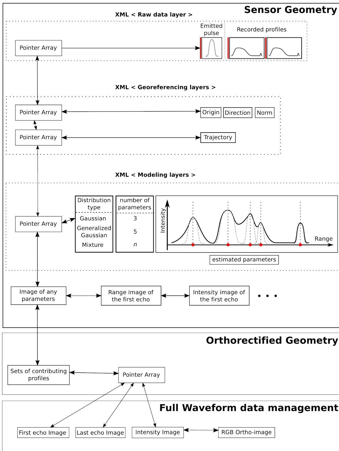
Figure 3: Sketch of the proposed data format for full waveform LiDAR data.
