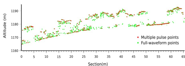
Figure 2: Profil of LiDAR points from multiple pulses data (red) and from full waveform data (green).
