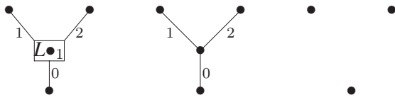
Figure 11: s -separability of the bipartite graph corresponding to a proof net
