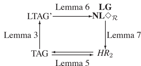
Figure 10: A summary of the previous lemma’s
